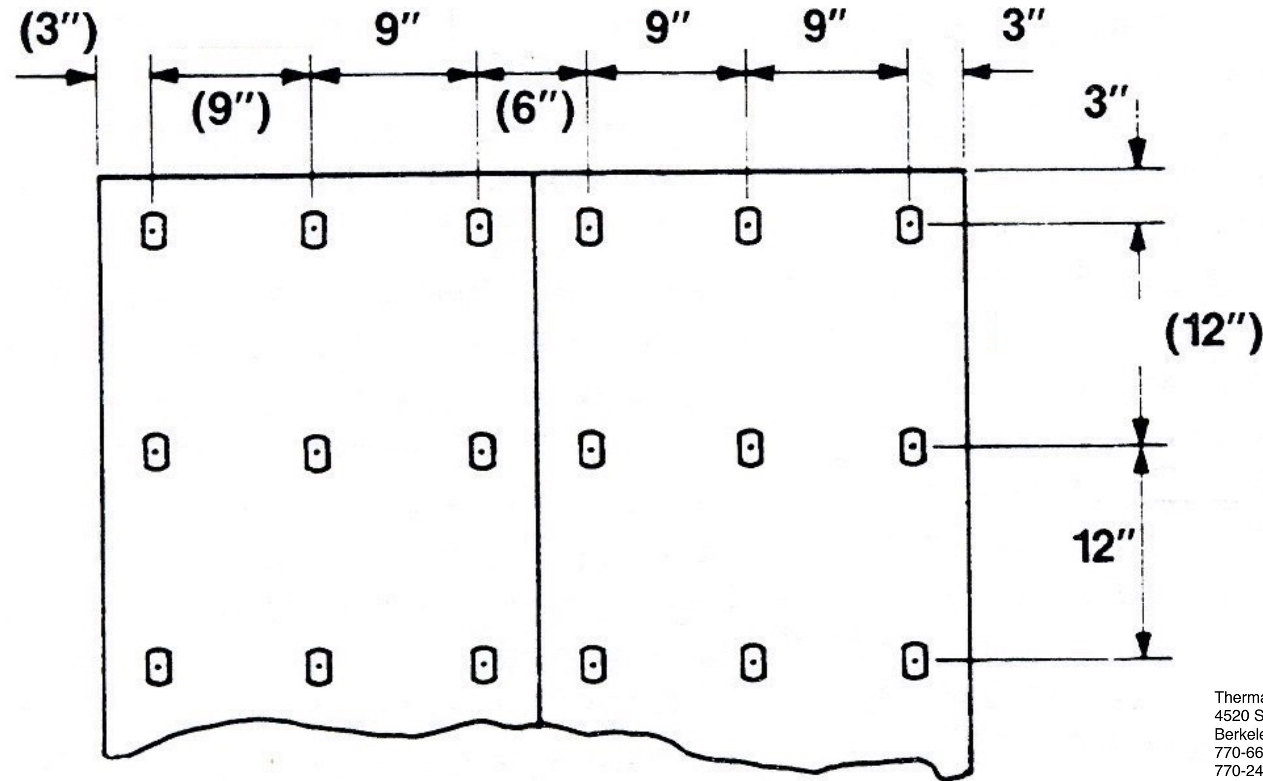
Walls— (1.5 Studs/ft 2 )
