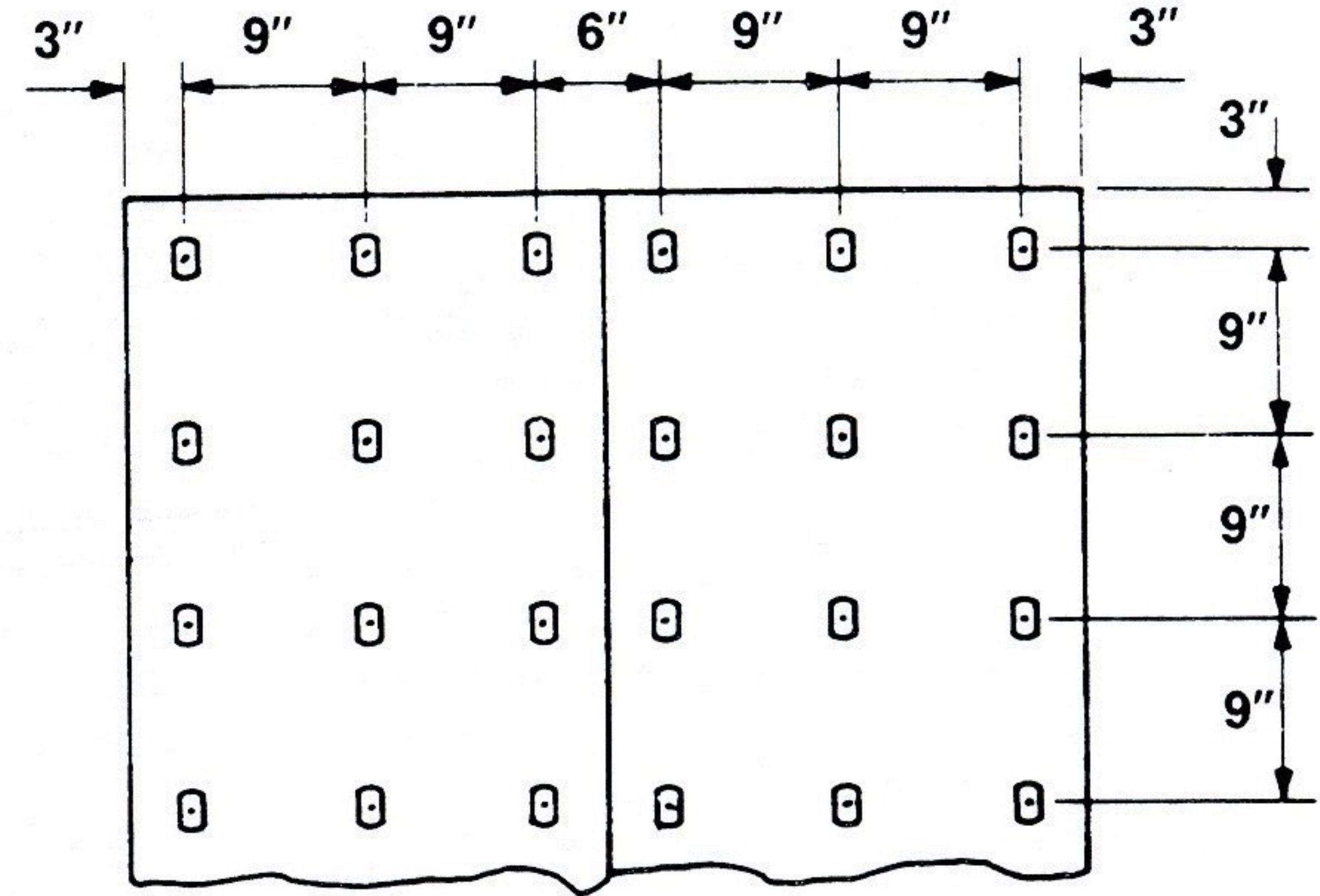
Roof— (2 Studs/ft 2 )
